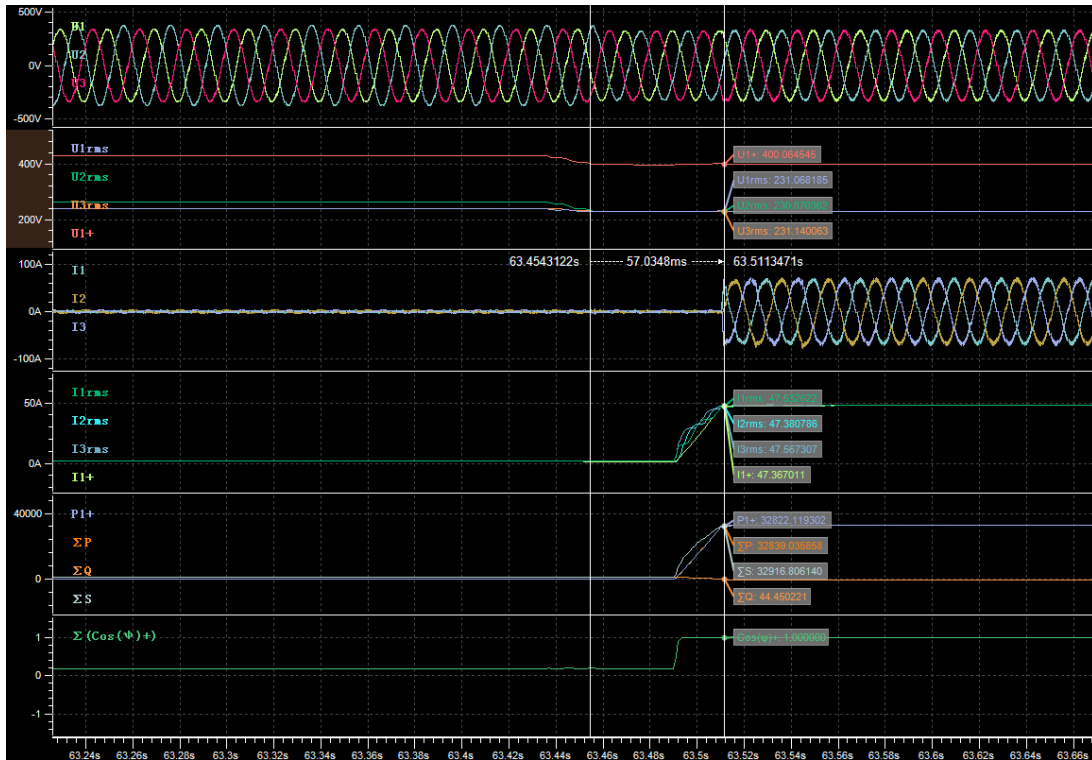
Recovery time
