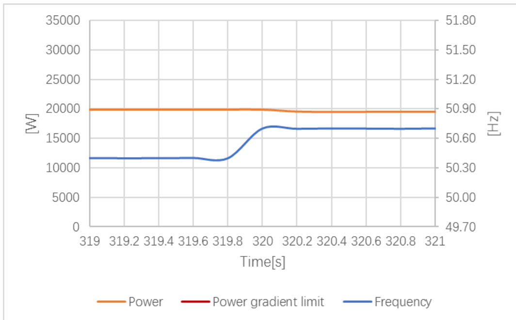
Response time
