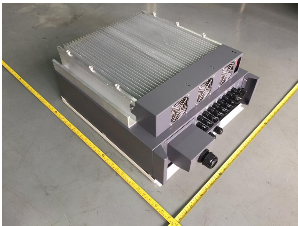
Rear view of model SOFAR 30000TL, SOFAR 33000TL
