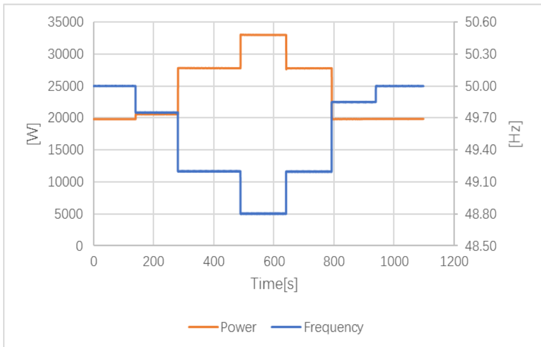
Test 2 P&F curve
