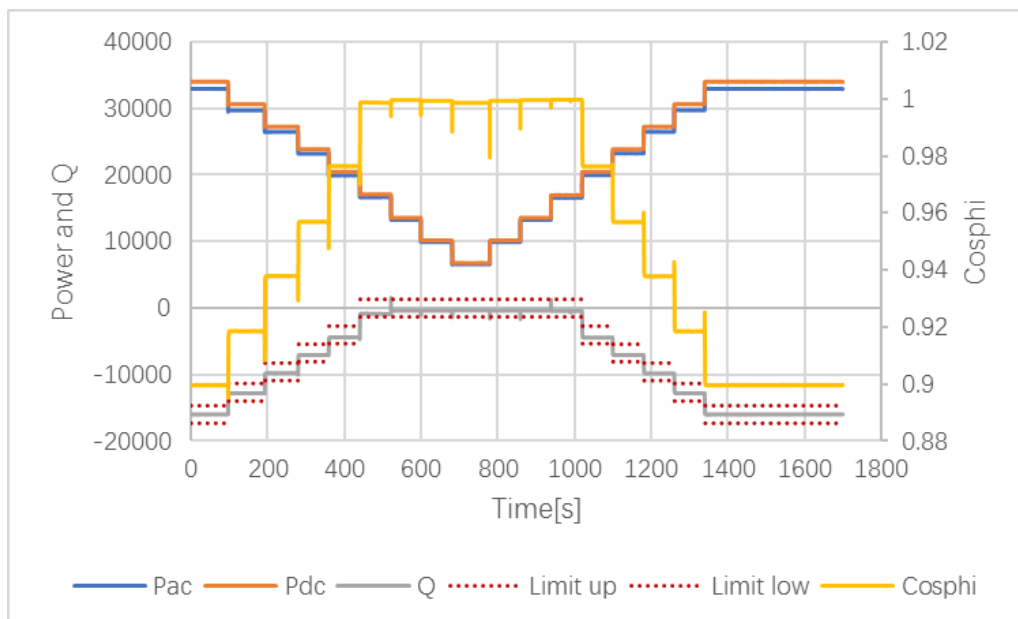
P(t), Q(t), Q set (t), Cosφ(t), tolerance(t) Diagram
