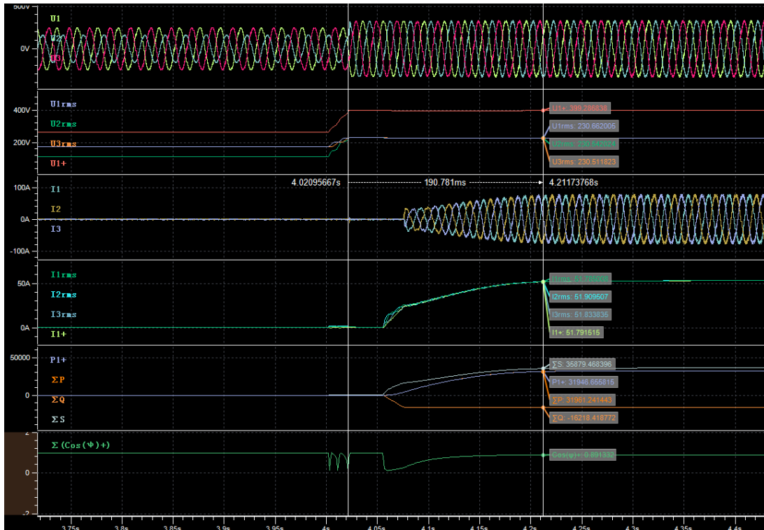
Recovery time
