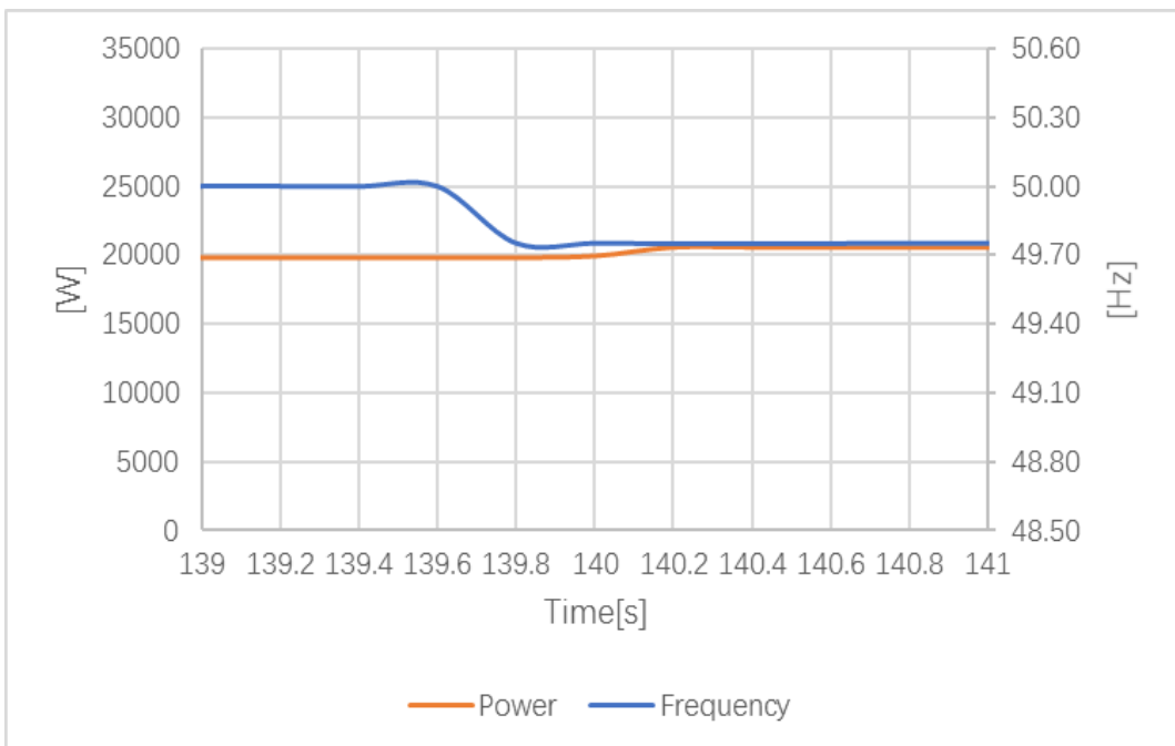
Response time
