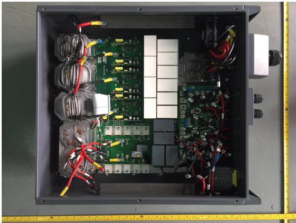
Internal view of SOFAR 30000TL, SOFAR 33000TL
