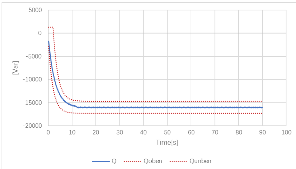
Q(t), Q set (t), tolerance(t) Diagram
