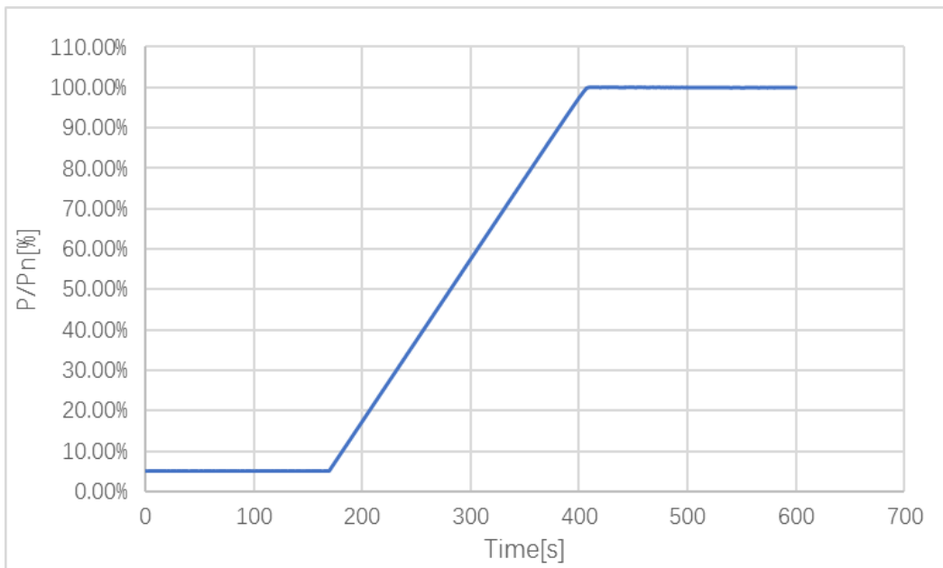
Power gradient from 5% to 100%
