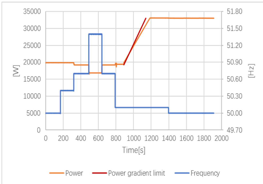
Test 2 P&F curve
