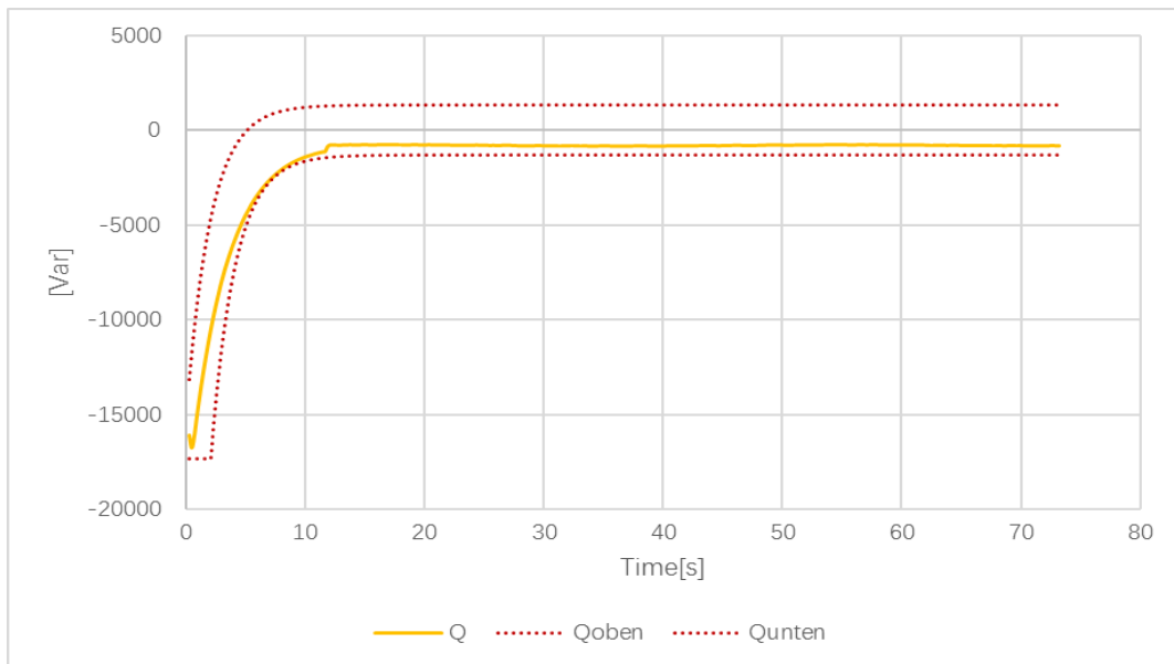
Power from 100% to 40% with PT1 character
