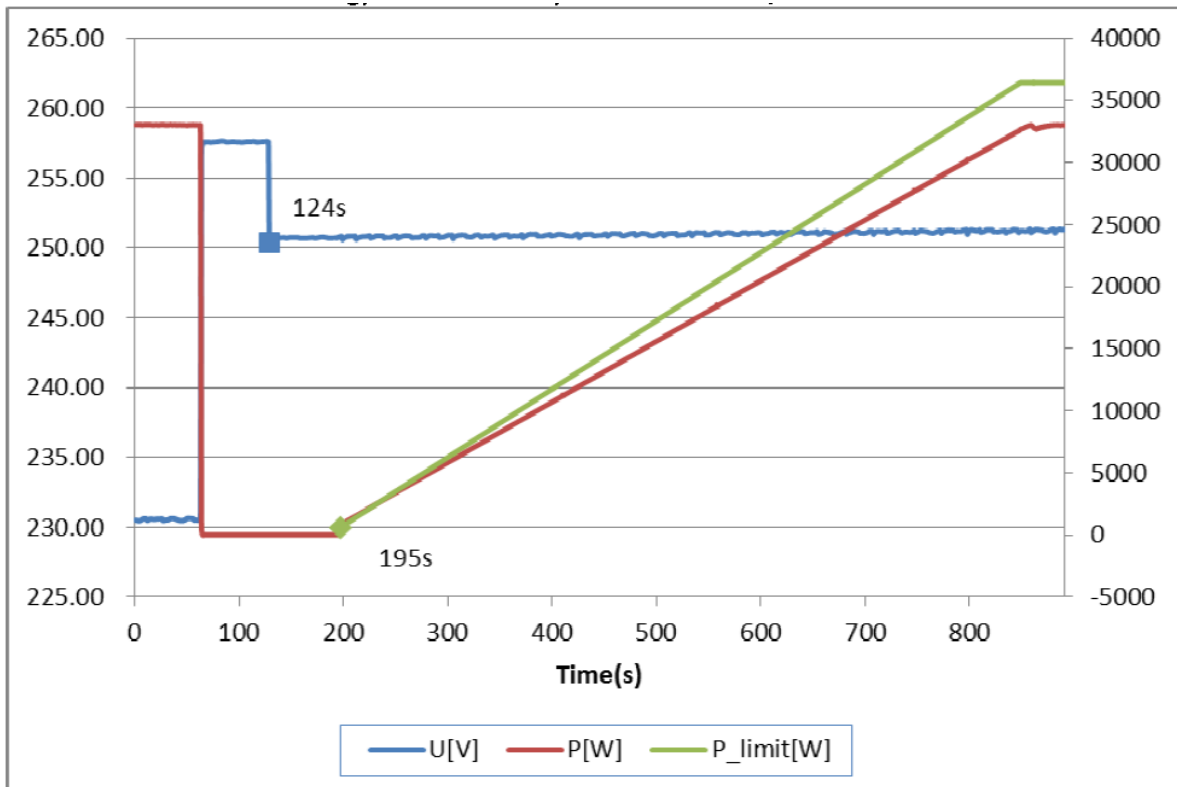
Graph of the gradual power supply and reconnection: for 109%Un
