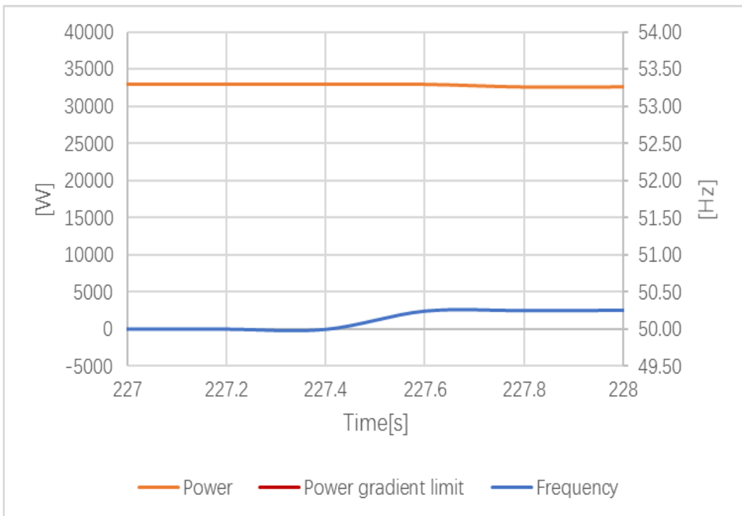
Response time
