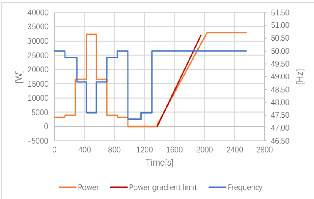
Test 1 P&F curve
