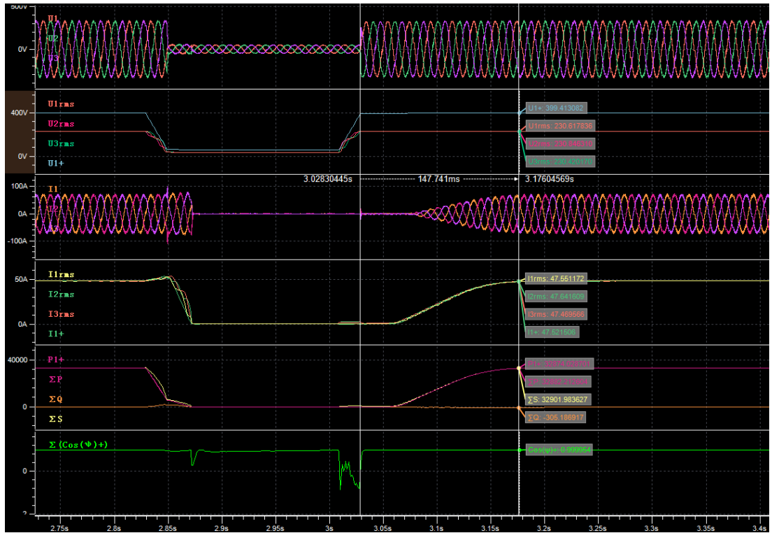
Recovery time
