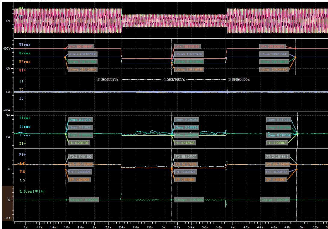
Empty load
