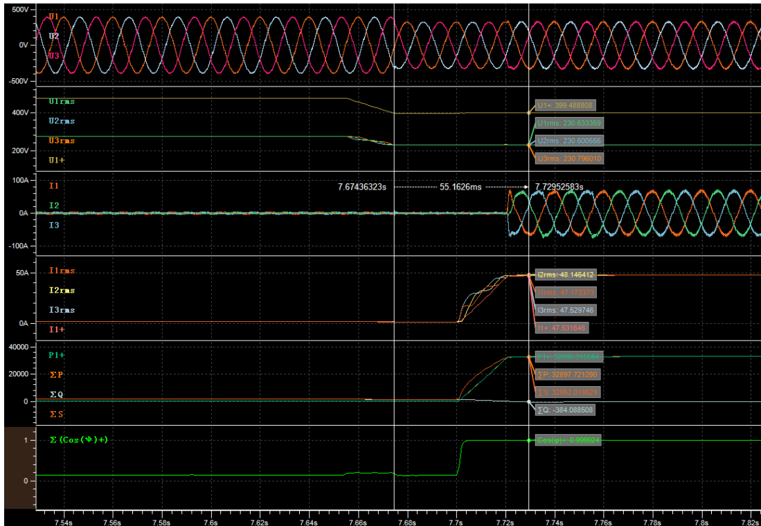
Recovery time
