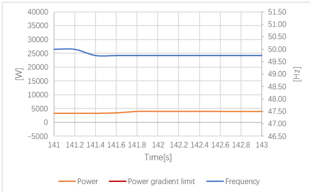
Response time
